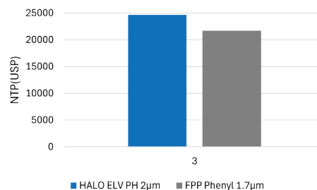
NTP Advantage Using HALO® vs. FPP Phenyl-Hexyl
